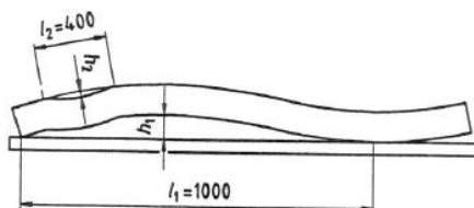
Figure 1 - Measurement of straightness from EN 12449:1999
